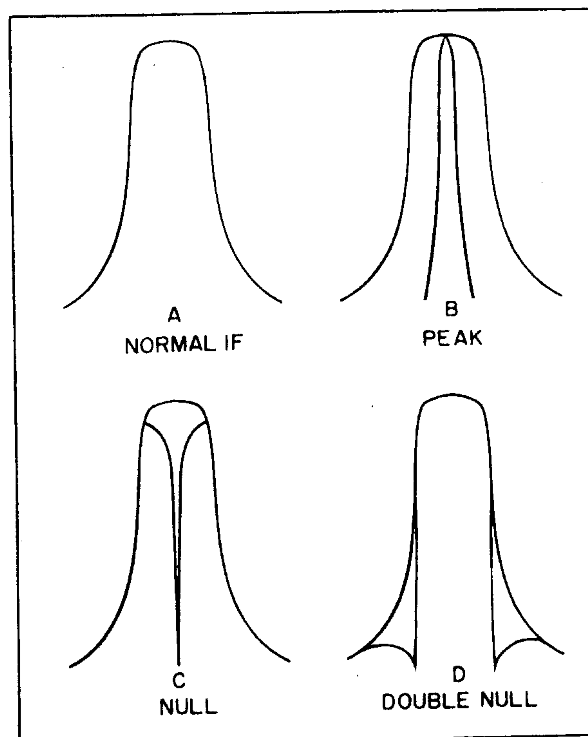
Figure 8. Q Multiplier Representative Curves
