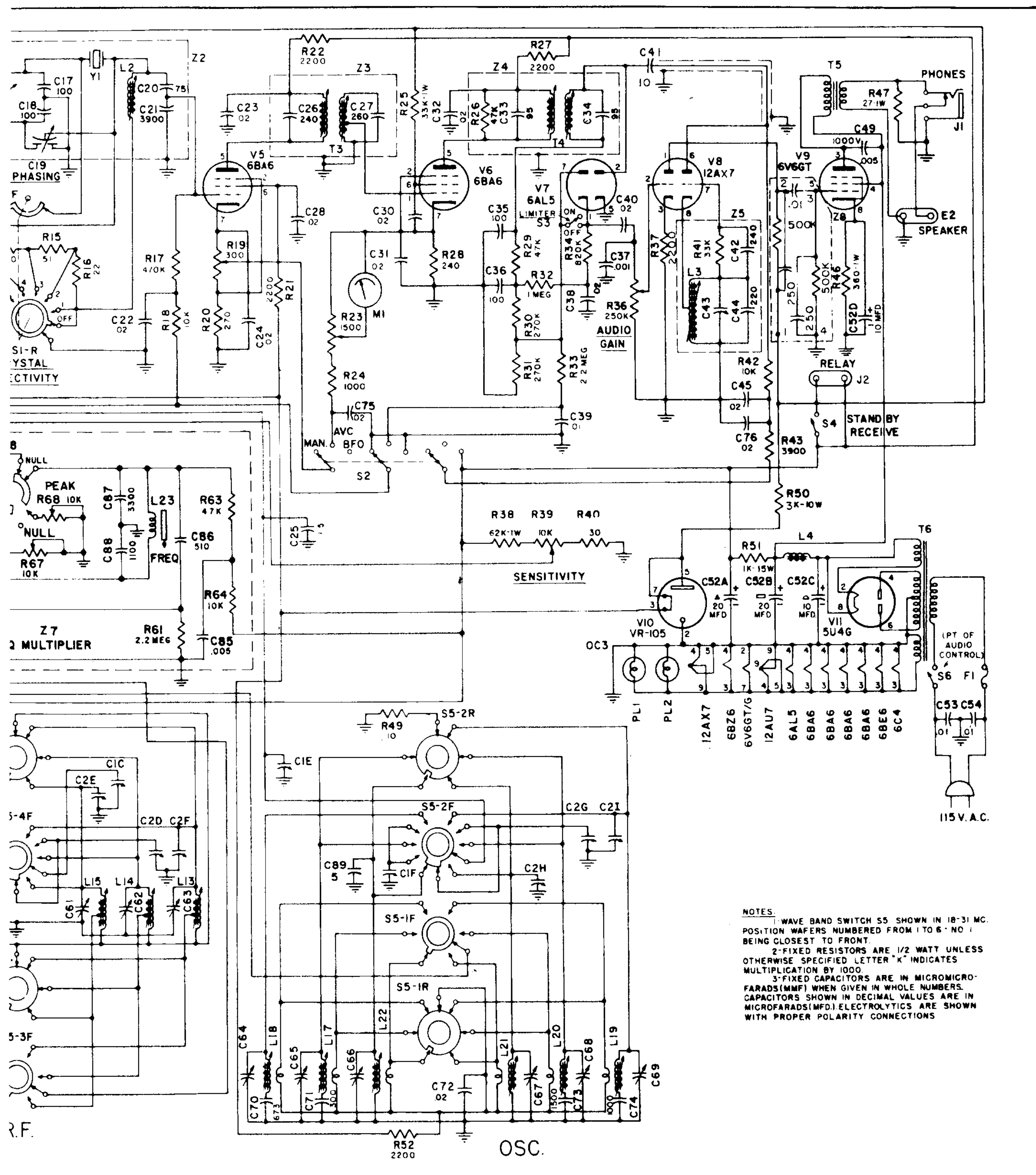
Figure 13. Hammarlund HQ-150 Receiver, Schematic Diagram
