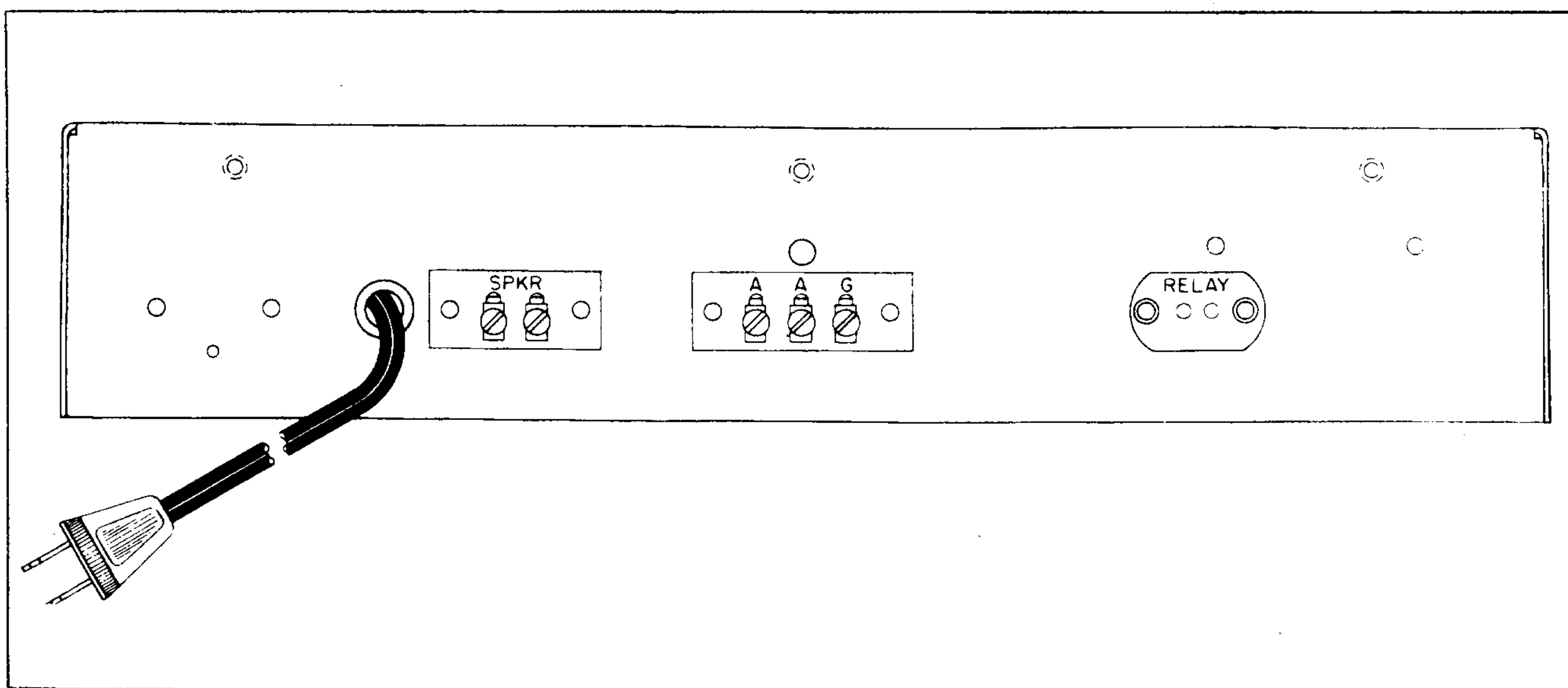
Figure 4. Connection Points at Rear of Chassis
