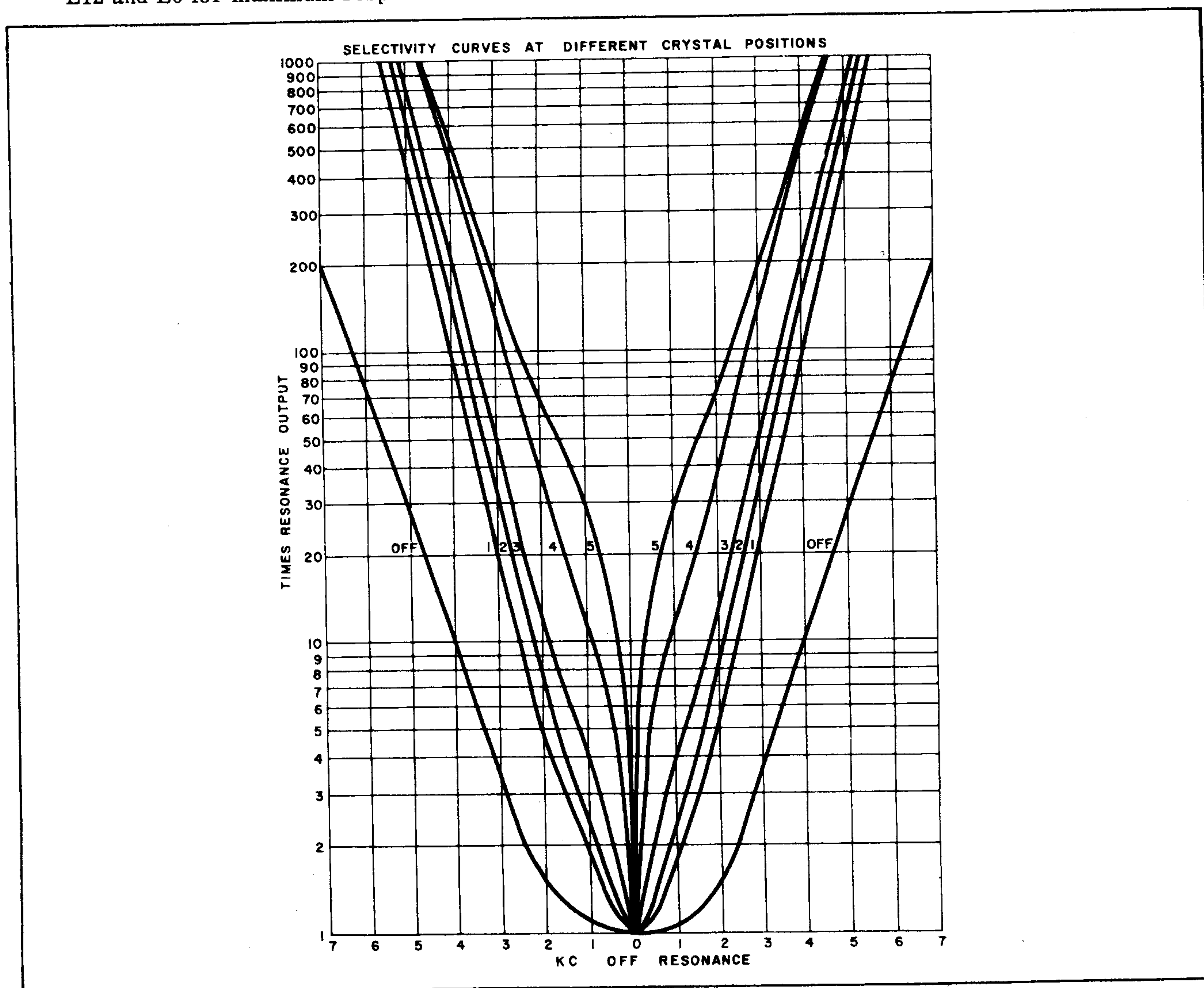
Figure 12. Selectivity Curves
